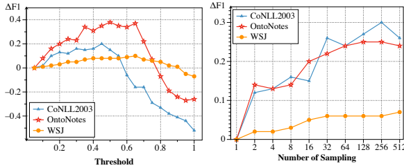
Figure 4: F1 variation under different uncertainty thresholds and numbers of sampling in variational LSTM, respectively. The results are evaluated on the development sets. \Delta F1 represents the F1 scores at different steps minus the initial results.
